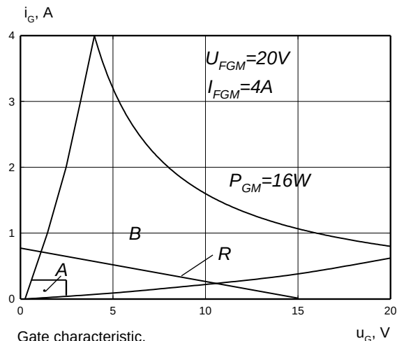
Gate characteristic.
