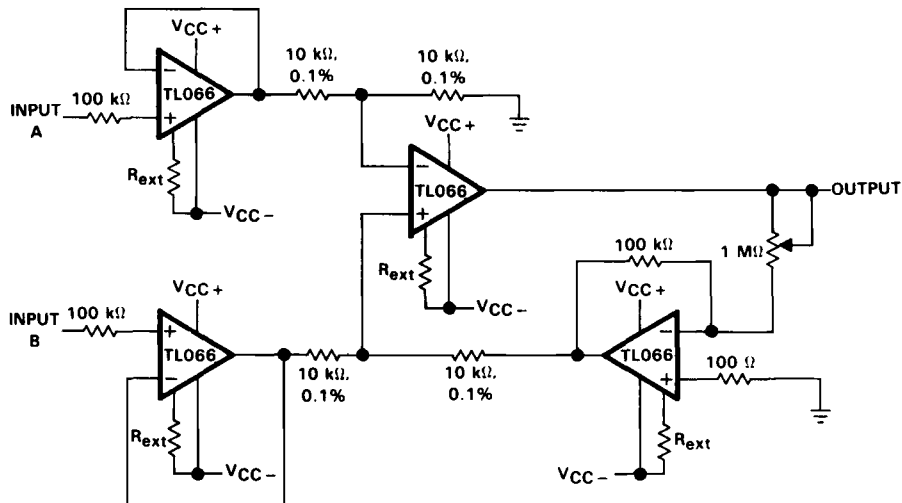
FIGURE 26. INSTRUMENTATION AMPLIFIER
