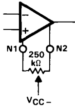
FIGURE 3. INPUT OFFSET VOLTAGE NULL CIRCUIT
