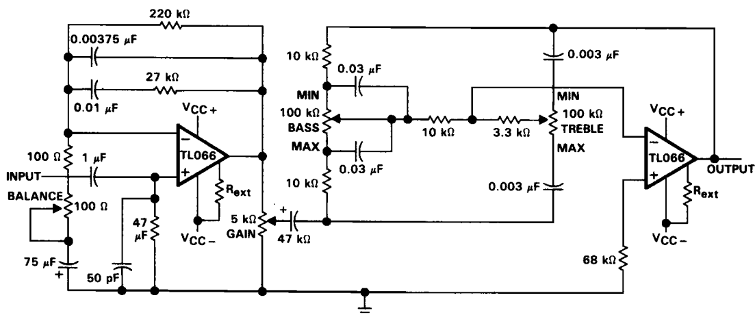
FIGURE 30. IC PREAMPLIFIER
