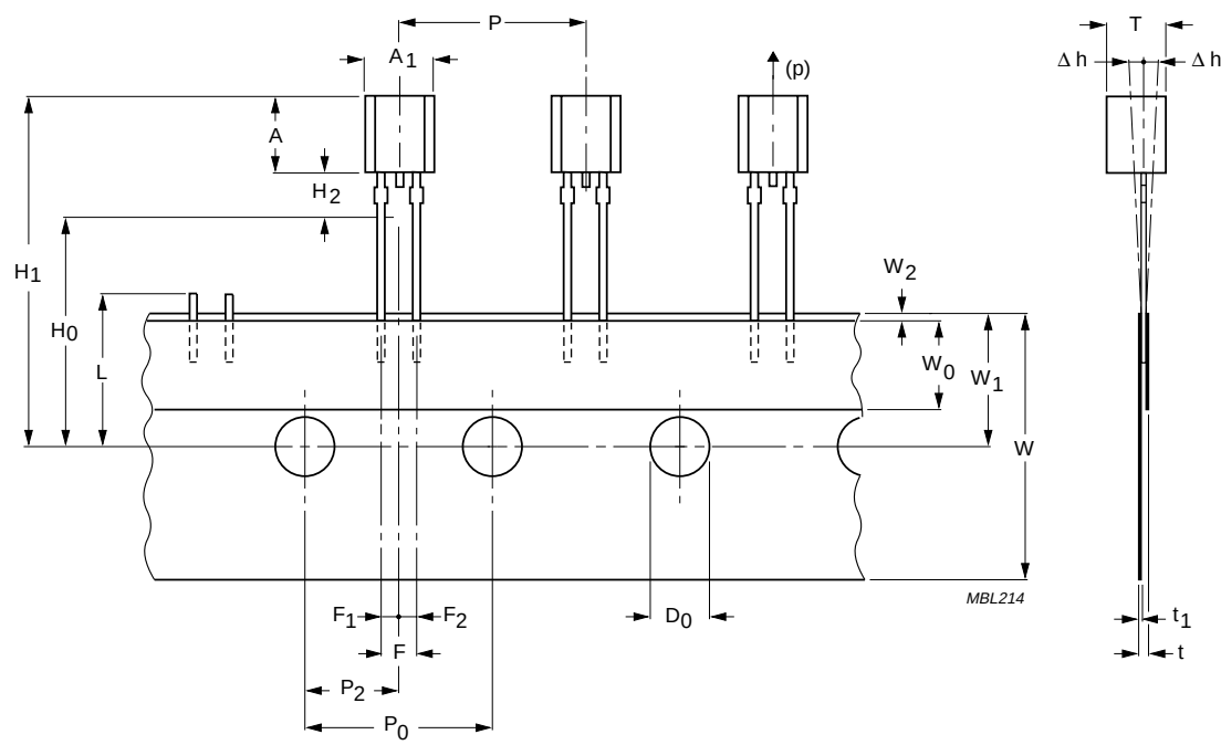
Fig.8 Configuration of bandolier: straight leads.
