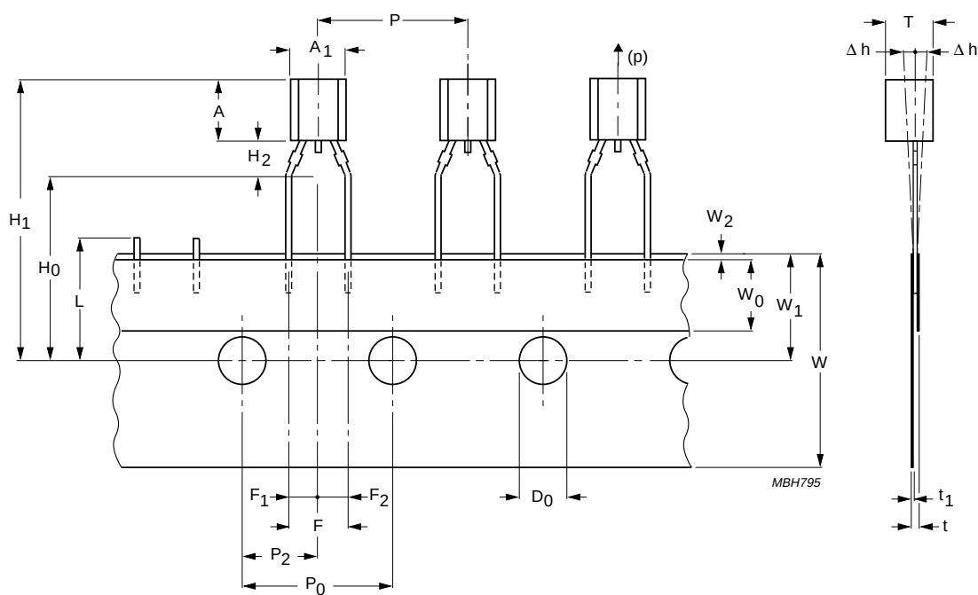
Fig.7 Configuration of bandolier: spread leads.
