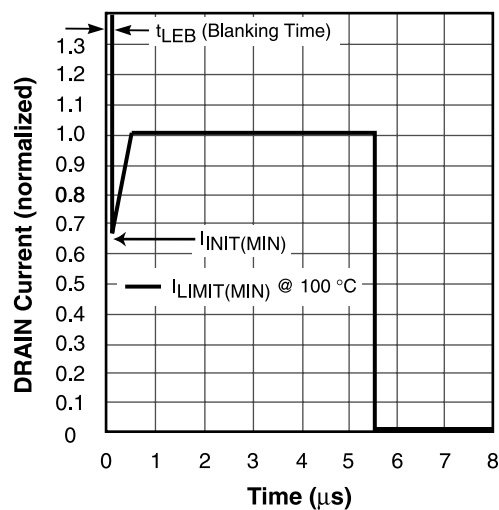
Figure 21. Current Limit Envelope.
