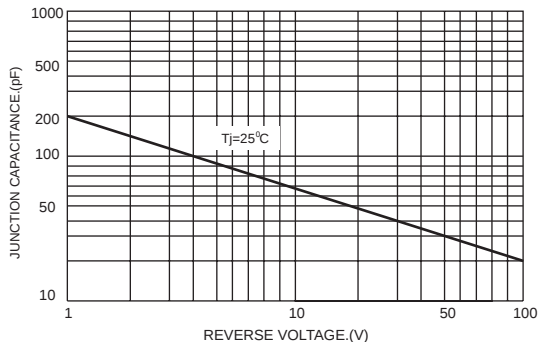
FIG.5-TYPICAL JUNCTION CAPACITANCE
