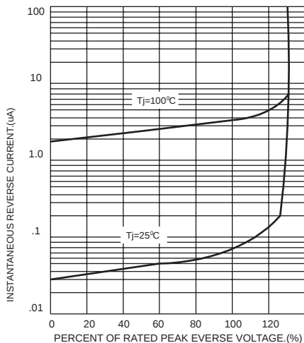
FIG.3-TYPICAL REVERSE CHARACTERISTICS
