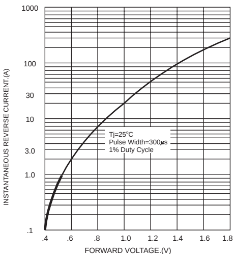
FIG.2-TYPICAL FORWARD CHARACTERISTICS
