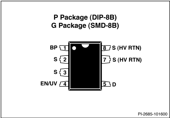
Figure 3. Pin Configuration.
