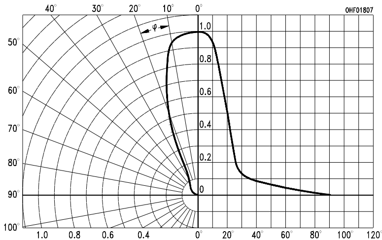
Directional Characteristics
