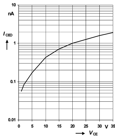
Dark Current
