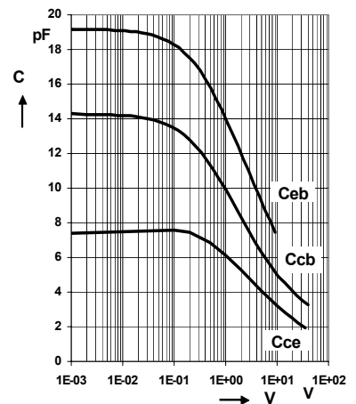
Capacitance
