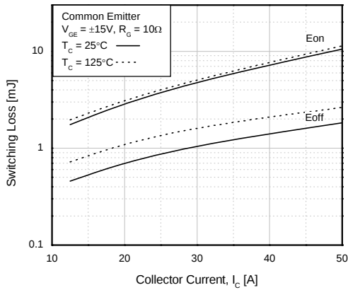
Figure 13. Switching Loss vs. Collector Current
