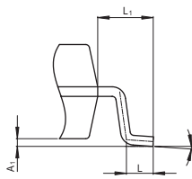
Detail F
