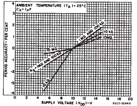
Fig. 11—Typical astable oscillator or Q, \overline{Q} period accuracy vs. supply voltage.
