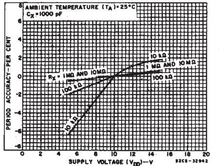
Fig. 13—Typical astable oscillator or Q, \overline{Q} period accuracy vs. supply voltage.
