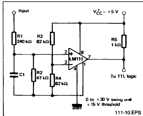
TTL INTERFACE WITH HIGH LEVEL LOGIC
