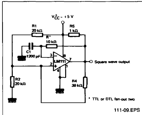
100kHz FREE RUNNING MULTIVIBRATOR
