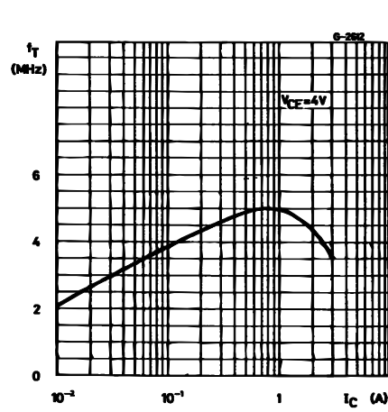
Transition Frequency (NPN type)
